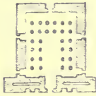
FIG. 110.—Portico in the Temple of Khons.
