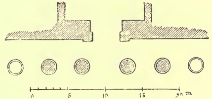
FIG. 113.—Portico in front of the façade of the temple of Gournah. From the Description , ii. 41.
