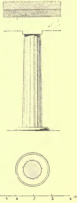
FIG. 73.—Sixteen-sided pillar; fluted.
