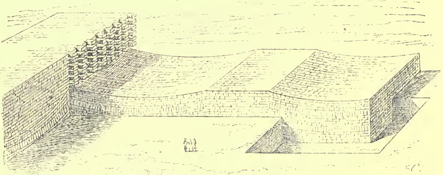
FIG. 50.—Foundations with inverted segmental arches ; compiled from Prisse.
